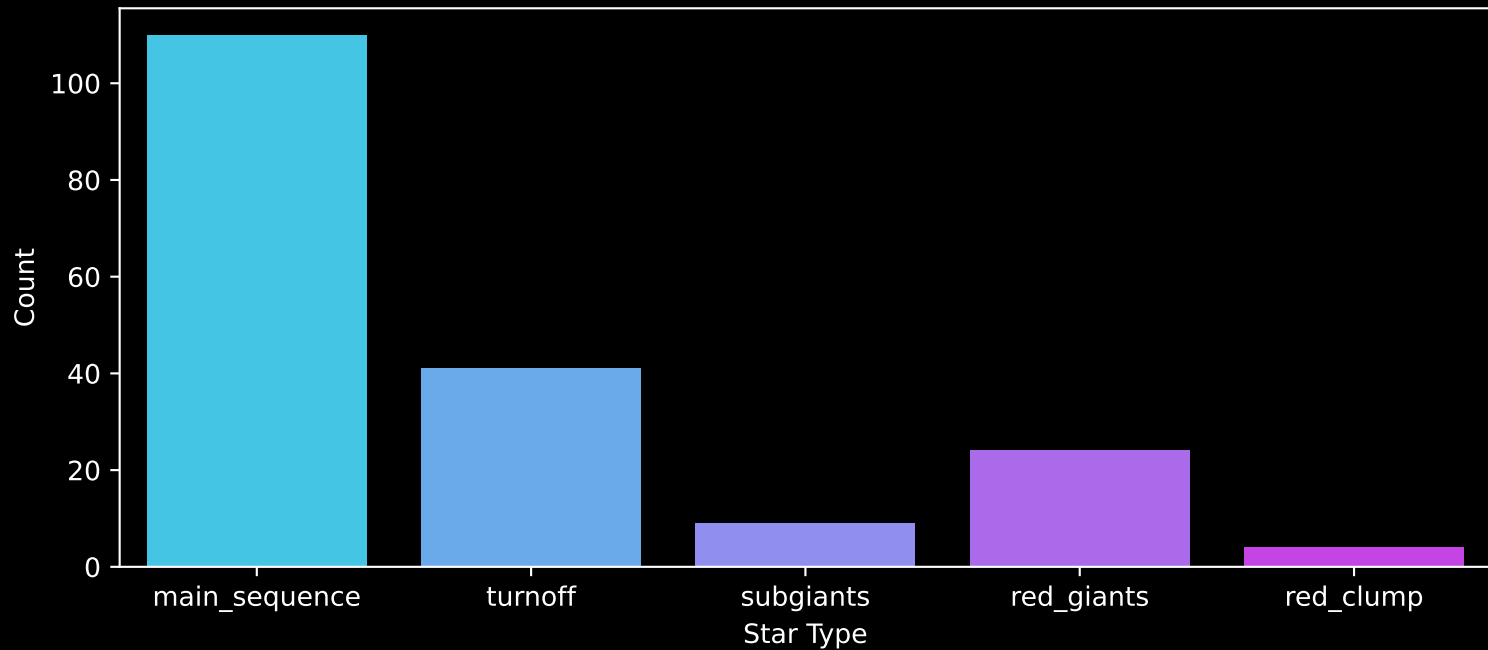
APOGEE DR17 Field: [154+62_MGA] Count plot of Star Type
