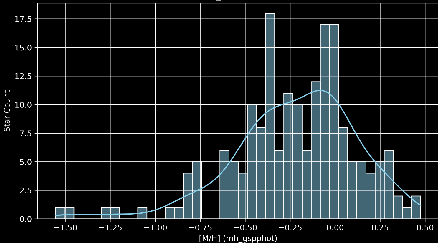
APOGEE DR17 Field: [154+62_MGA [M/H] (mh_gspphot) (n= 184)
