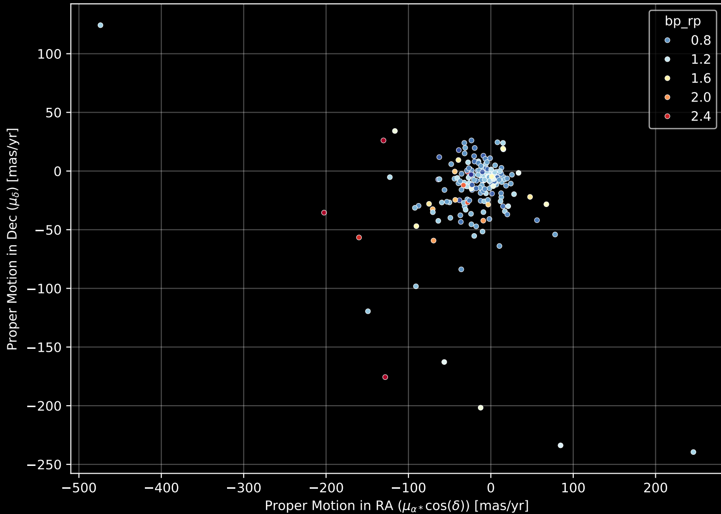
APOGEE DR17 Field: [154+62_MGA] Proper Motion Diagram (n= 188)
