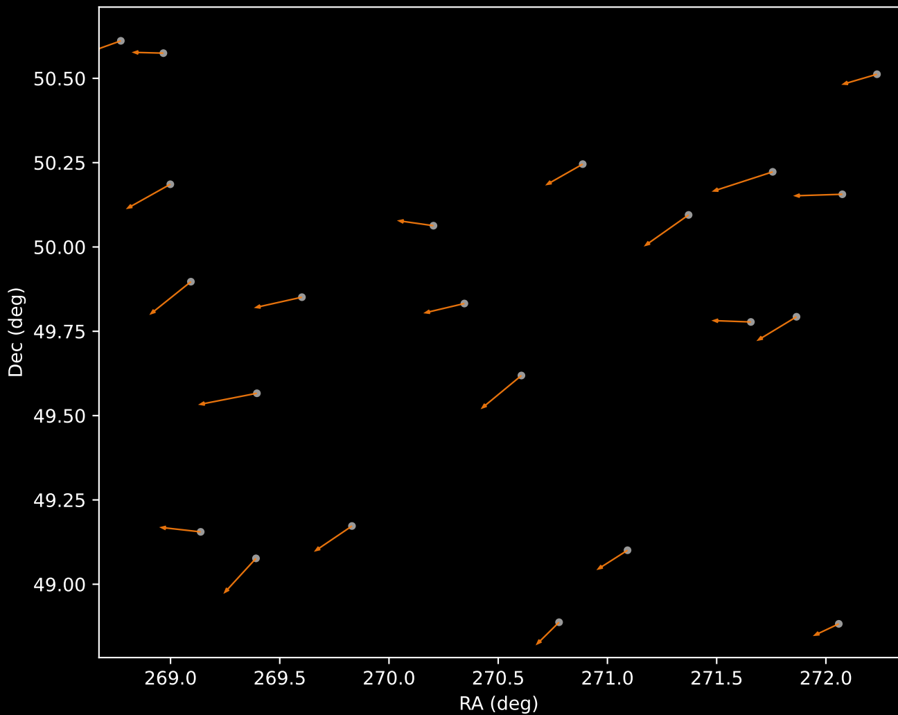
APOGEE DR17 Cluster 2 Proper Motion Vectors (n=22)
