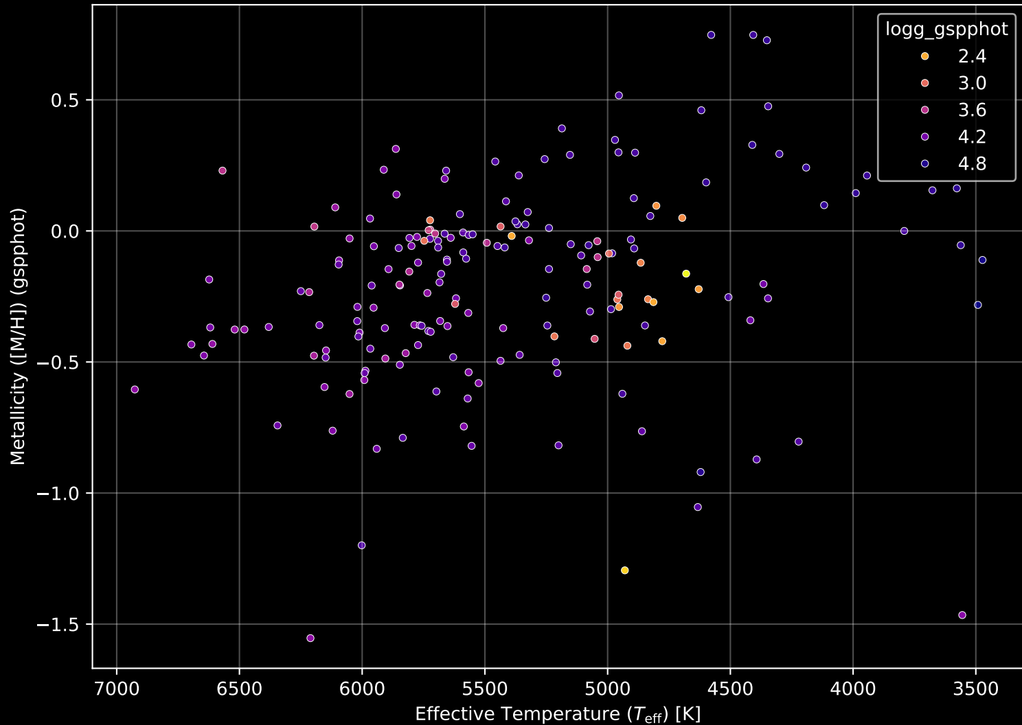
APOGEE DR17 Field: [154+62_MGA] Stellar Population Parameters (n= 188)
