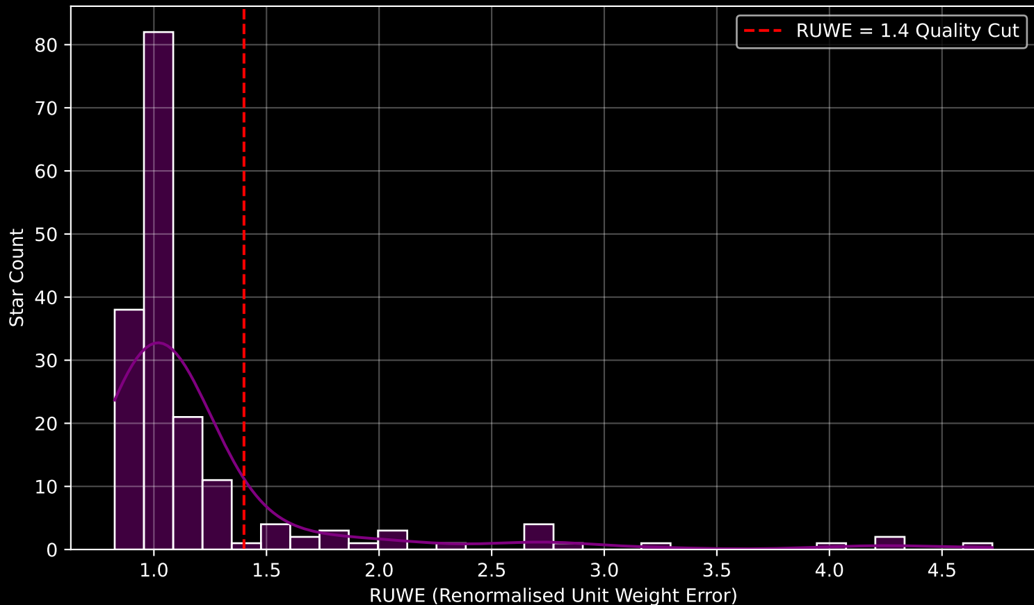
GAPOGEE DR17 Field [154+62_MGA] RUWE Distribution (n= 177)
