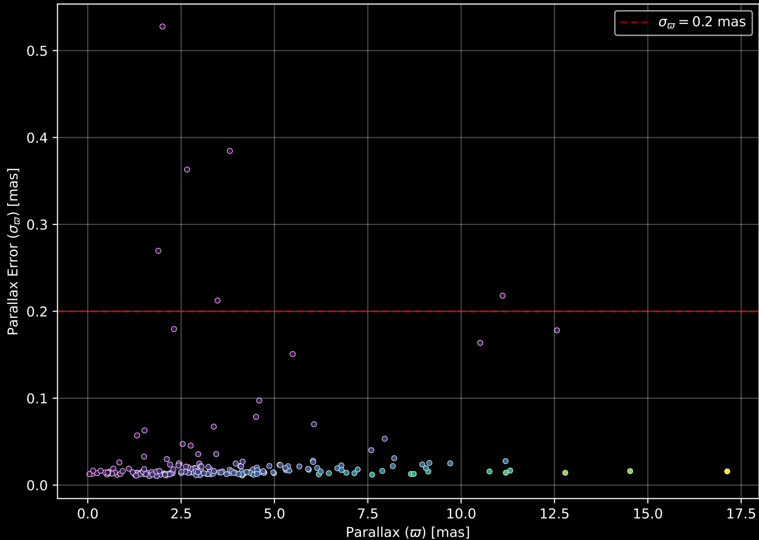
APOGEE DR17 Field: [154+62_MGA] Parallax Quality (n= 188)
